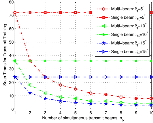
Fig. 3. Performance comparison between the proposed multi-beam transmit training and the traditional solution.
