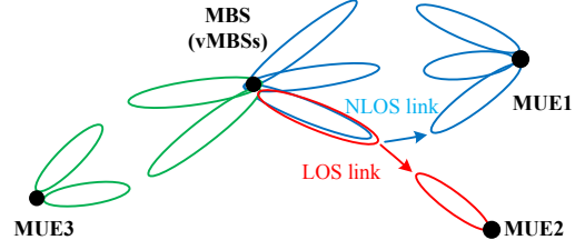
Fig. 1. An example of 2D view of beamspace MU-MIMO ( U = 3 ). Note that, in order to make the figure clear, we do not show the side lobes here.
