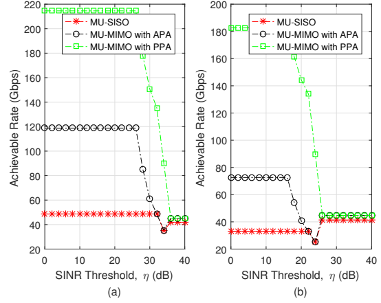
Fig. 4. Achievable rate performance versus SINR threshold \eta for beam-space MU-SISO and MU-MIMO with PPA and with APA, respectively, given that \xi_t = 10^\circ , \xi_r = 15^\circ , and (a) z = 0.01 , (b) z = 0.1 .
