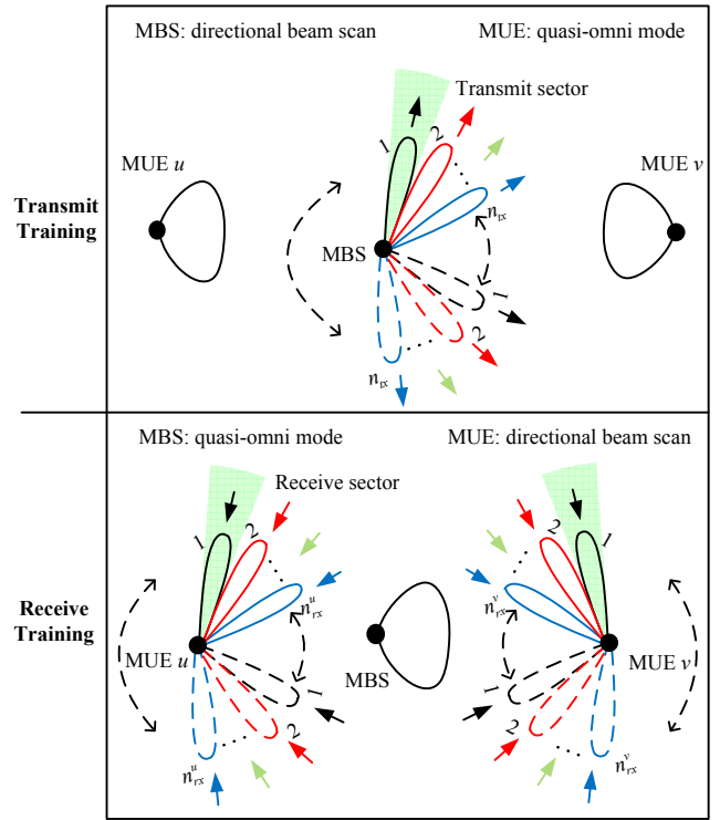
Fig. 2. Illustration of transmit and receive training for downlink beamspace MU-MIMO, given that U_{\text{total}} = 2 . The beams drawn with solid lines are operated concurrently and it is the same to that drawn with dotted lines.
