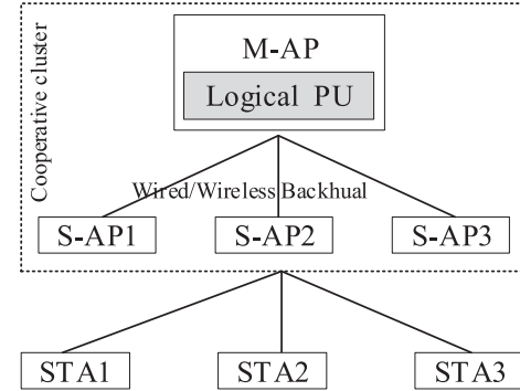
Fig. 14. An example of the multi-AP architecture, where a group of APs are connected by wired or wireless links and the logical processing unit (PU) located at the M-AP is used to coordinate/control the related multi-AP operations of multiple distributed APs.
