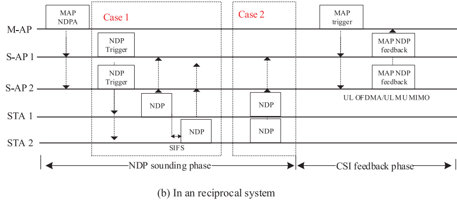
Fig. 16. Acquisition of CSI between the multiple APs and STAs in the non-reciprocal/reciprocal system. (a) In the non-reciprocal system, the coordinate AP (M-AP) first initiates the multi-AP sounding by sending the NDPA frame, then multiple S-APs will send NDP simultaneously/sequentially following the sequence specified in the NDPA frame, and finally the STAs feedback CSI in the OFDMA/UL MU-MIMO way. (b) In the reciprocal system, multiple STAs transmit NDP sounding frame simultaneously/sequentially in response to the soliciting NDP Trigger frame containing information indicating the timing at which the STAs respectively to transmit NDP sounding frames.
