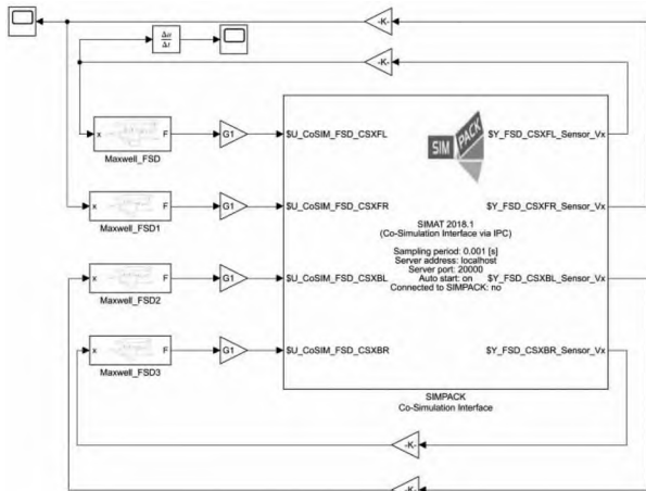
图9 Simpack-Simulink 联合仿真模型 Fig. 9 Simpack-Simulink co-simulation model
