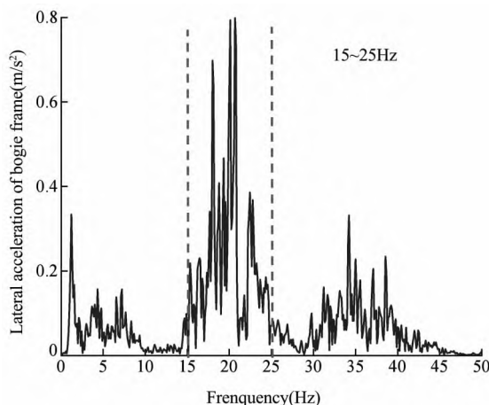
(a) 构架横移振动频谱图 (a) Spectrum diagram of bogie frame lateral displacement
