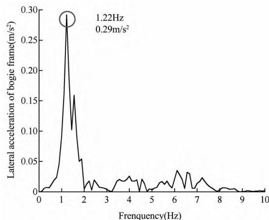
(b) 车体横移振动频谱图 (b) Spectrum diagram of car body lateral displacement
